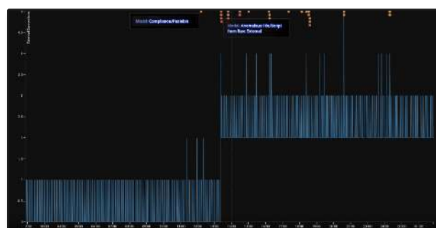
Figure 23: Graphical representation of the sudden increase in external connections and related model breaches
