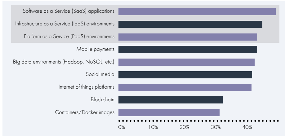
Figure 11 – Environments Used to Store Sensitive/Regulated Data Source: 2019 Thales Data Threat Report Survey, IDC, November 2018
